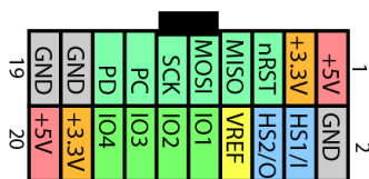
Connector View
